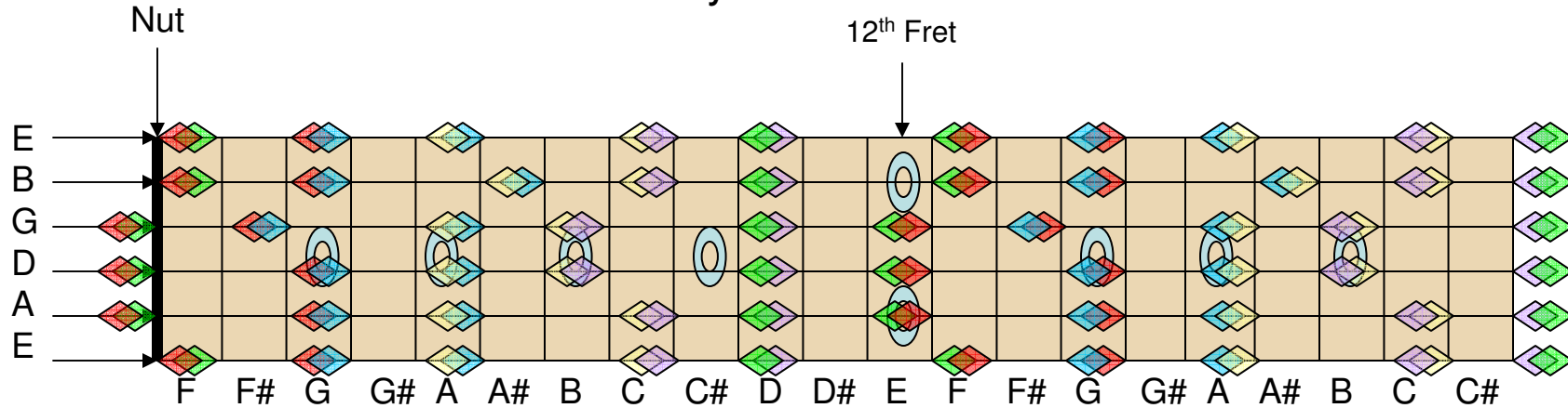
Key of D Entire Scale
