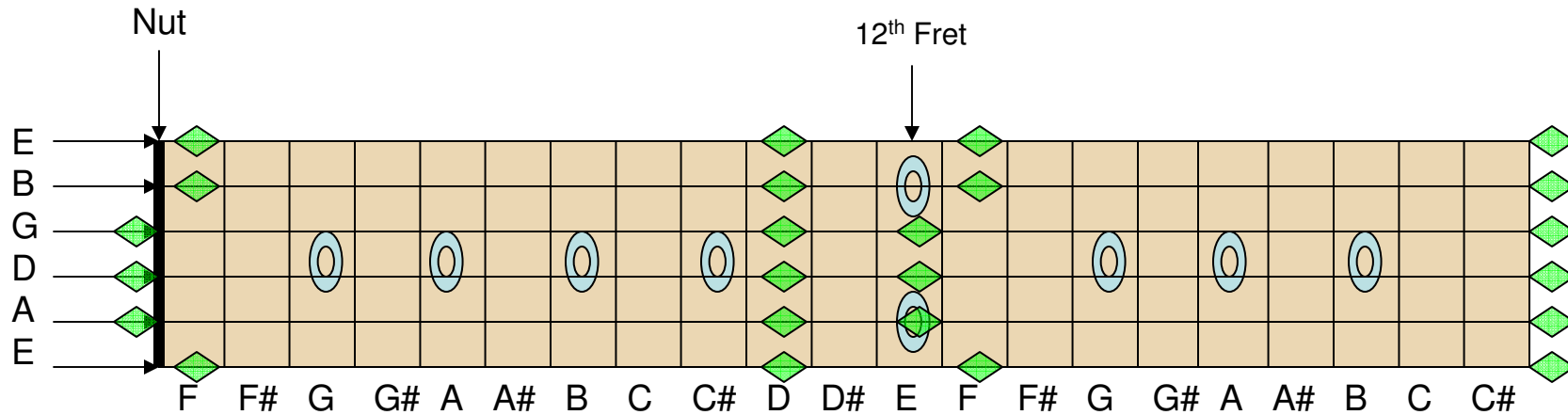
Key of D Root Pattern 1
